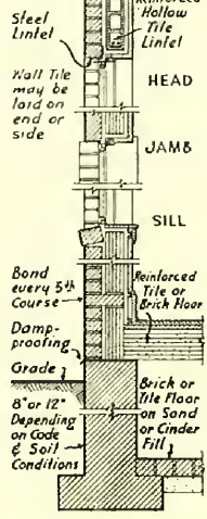
Wall Section
